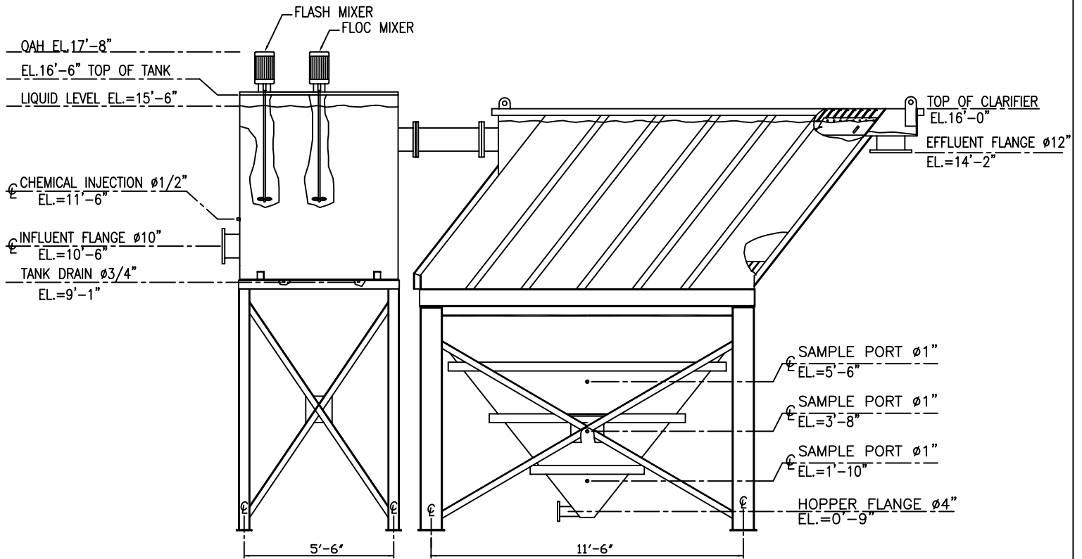
SIDE ELEVATION
